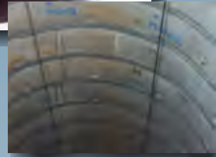
UTE Ave Túnel Serrano-Chamartín Joint Sealing of Emergency wells Resin injection.(8.000kg)
